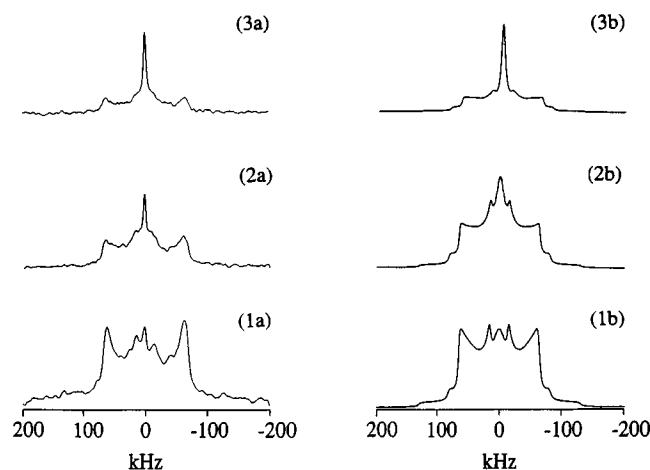
FIGURE 2 ^2\text{H} NMR spectra of polycrystalline carboxypeptidase A samples cross-linked with glutaraldehyde and soaked in a 10 mM solution of D-Phe-d5 obtained at 11.7 T at different water contents. The experimental conditions and the approach to the simulations were the same as in Fig. 1, except that k_2 = 1.1 \times 10^4 \text{ s}^{-1} and (2b) k_1 = 1.5 \times 10^6 \text{ s}^{-1} , and (3b) k_1 = 1.9 \times 10^6 \text{ s}^{-1} .
