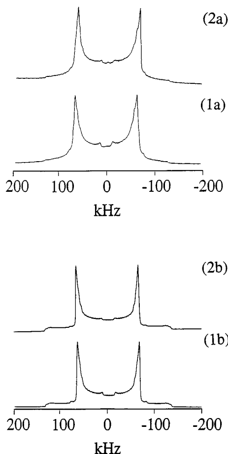
FIGURE 8 ^2\text{H} NMR spectra of phenylacetic acid recrystallized slowly and measured at 11.7 T at 298 K. Spectra were obtained using approximately 100-mg samples, 512 transients, and a recycle delay of 100 s. The deuterium quadrupole-echo delays were (1a) 35 \mu\text{s} , (2a) 150 \mu\text{s} . The corresponding simulated spectra (1b, 2b) were obtained assuming three pairs of two-site jumping motions for the phenyl ring about the C-2 axis with the same jumping rate of 9.4 \times 10^4 \text{ s}^{-1} , a quadrupole coupling constant of 178 kHz, \eta = 0.0 , line broadening of 1 kHz, and 2048 points in the spectral array. The three pairs of two sites have orientations with respect to the C-2 axis of the phenyl ring and populations, (0°, 60°, 0°) and (24°, 60°, 0°), p_1 = p_2 = 0.5 ; (0°, 60°, 0°) and (34°, 60°, 0°), p_1 = p_2 = 0.5 ; (0°, 60°, 0°) and (73°, 60°, 0°), p_1 = p_2 = 0.5 . The spectral weight factors for the three pairs are 1:1:2.
