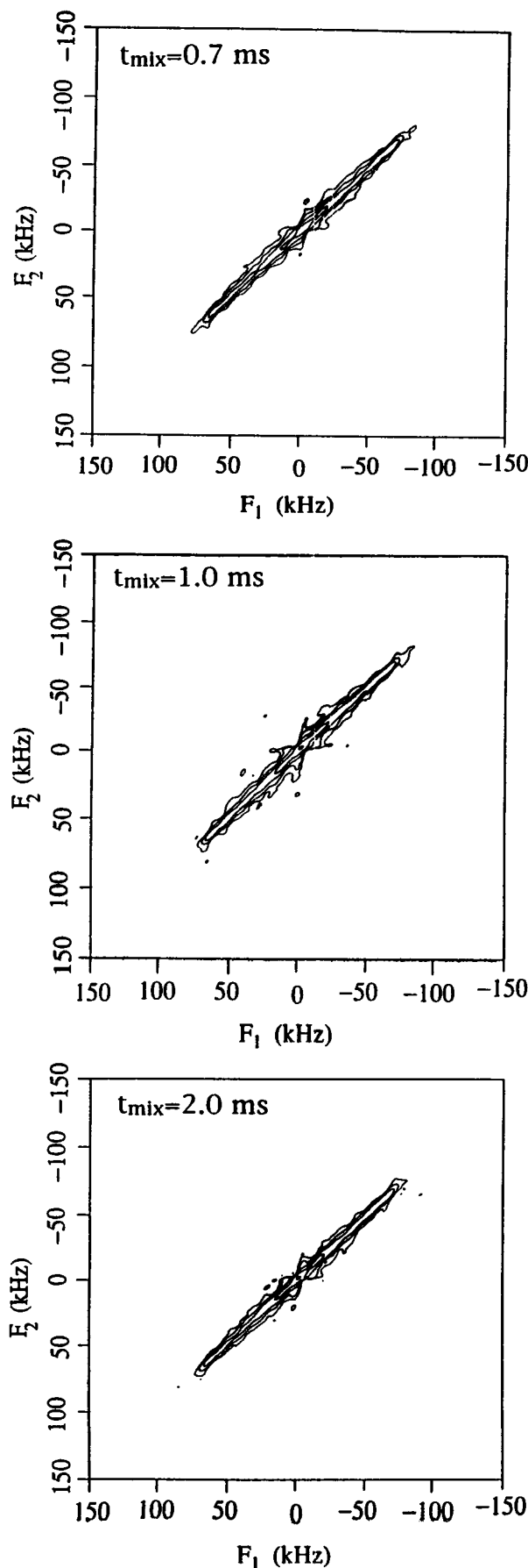
FIGURE 6 Two-dimensional ^2\text{H} NMR exchange spectra for polycrystalline carboxypeptidase A samples cross-linked with glutaraldehyde and soaked in 10 mM PPA- d_5 obtained at 11.7 T at a relative humidity of 81%. Spectra were obtained with approximately 200-mg samples, 8192 transients, a recycle delay of 0.5 s, an echo delay of 35 \mu s, and mixing times of (a) 0.7 ms, (b) 1 ms, and (c) 2 ms.
