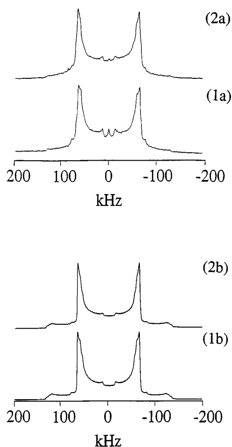
FIGURE 9 ^2\text{H} NMR spectra of polycrystalline phenylacetic acid recrystallized slowly, obtained at 11.7 T and 315 K. Experimental conditions were the same as summarized in Fig. 8, except that 256 transients were collected. The simulated spectra (1b, 2b) were obtained with a ring jump rate of 1.9 \times 10^5 \text{ s}^{-1} .
