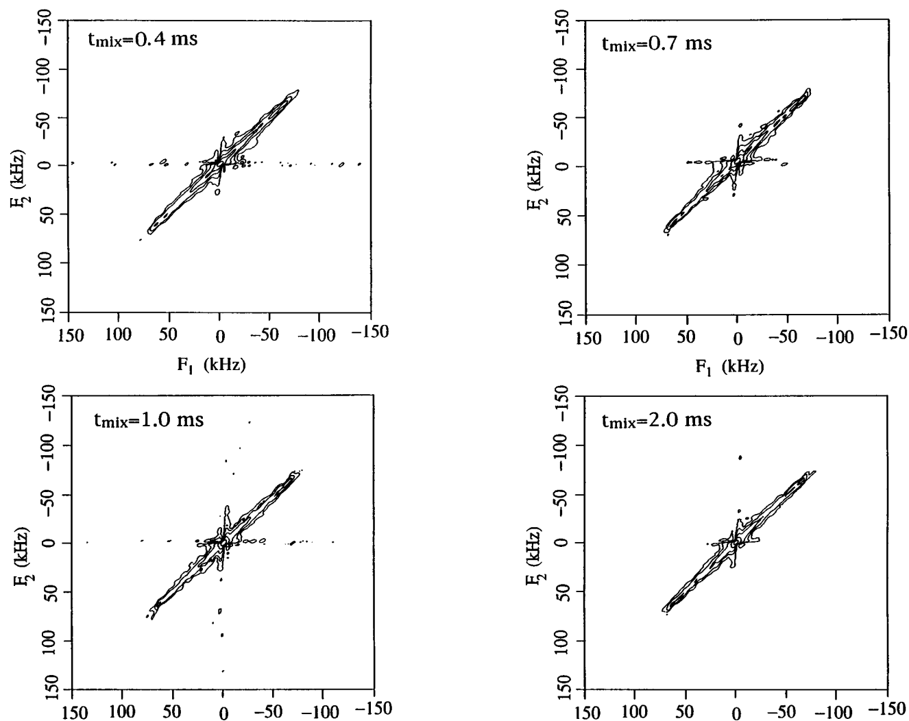
FIGURE 7 Two-dimensional ^2\text{H} NMR exchange spectra of polycrystalline carboxypeptidase A samples cross-linked with glutaraldehyde and soaked in 10 mM PPA-d5 obtained at 11.7 T at a relative humidity of 98%. The experimental conditions were the same as in Fig. 6, except that the mixing times were 0.4 ms, 0.7 ms, 1 ms, and 2 ms.
